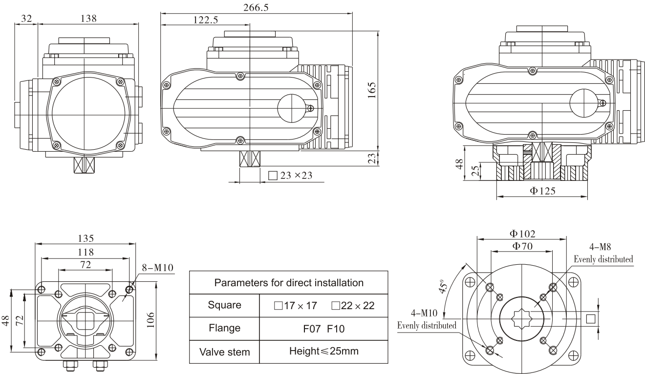
Explosion-proof standard type
